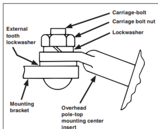
Figure 7. Attaching an overhead pole-top style VacuFuse II interrupter cutout mounting to the mounting bracket.
