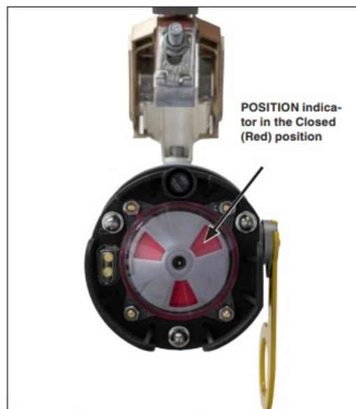
Figure 6. The vacuum interrupter in the Closed position.
