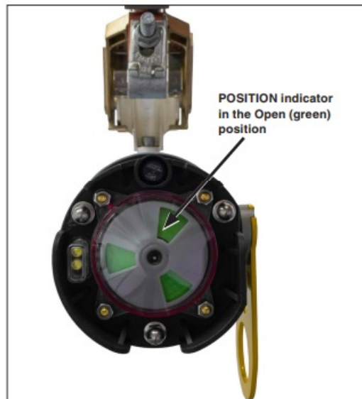
Figure 5. The vacuum interrupter in the Open position.
