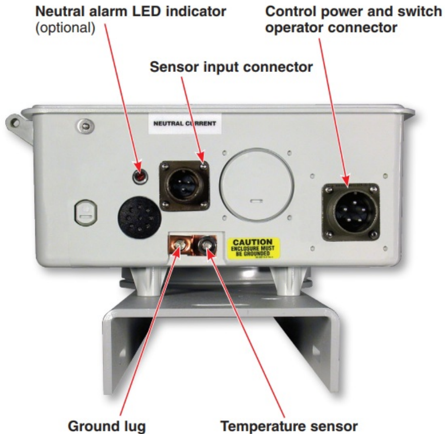
Figure 2. Underside of enclosure.
