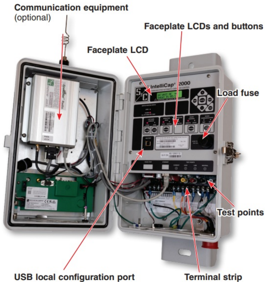
Figure 1. Interior of enclosure.
