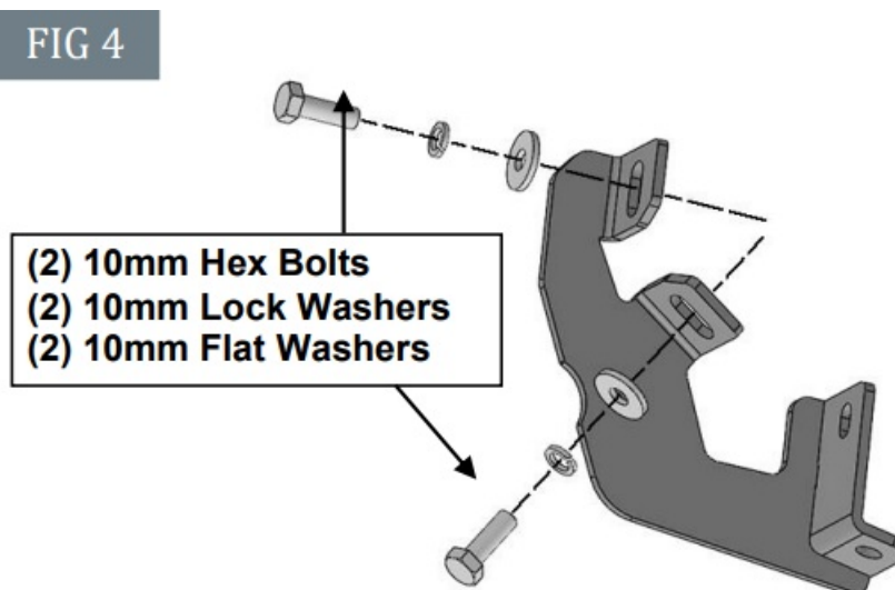
(Fig 4) Attach (1) Passenger/Right Rear Mounting Bracket to the rear location.
