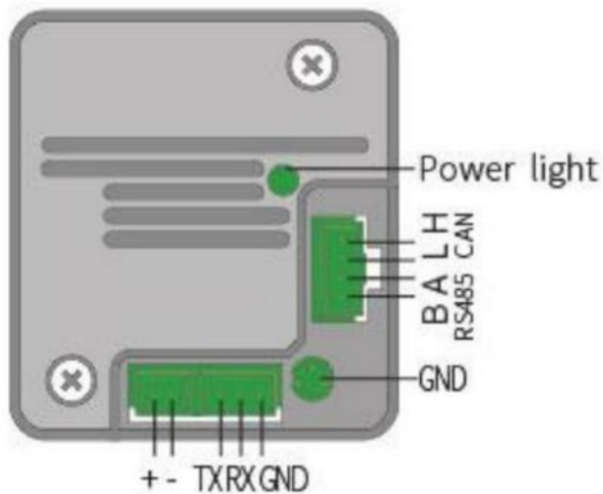
Figure 2-8 Port Definition of Driver Board
