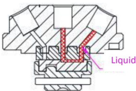
Figure 2-6-1 Dead volume (port to port)
