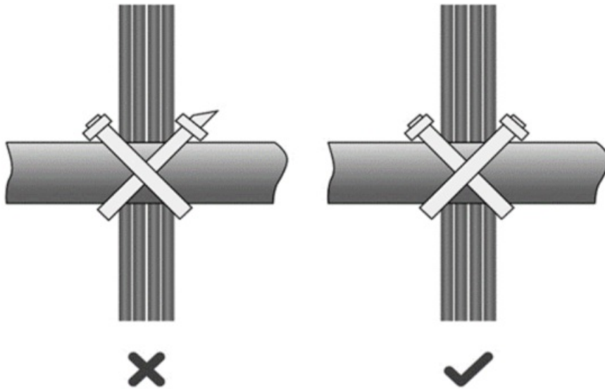
Figure 7-5 Bundling up Cables (2)
