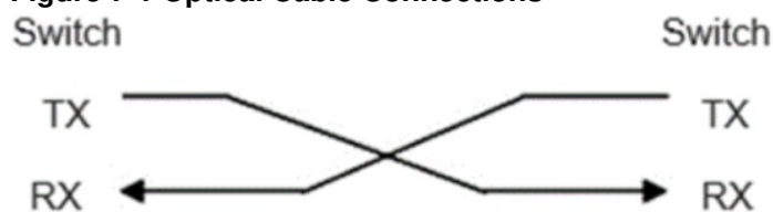
Figure 7-1 Optical Cable Connections
