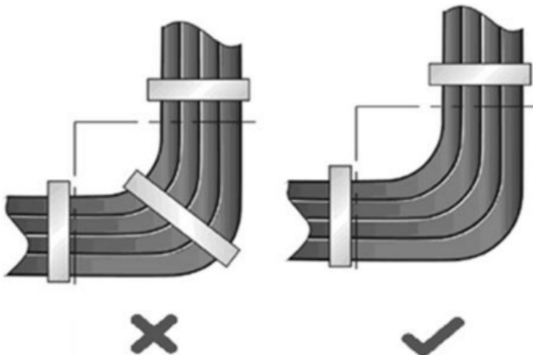
Figure 7-6 Bundling up Cables (3)
