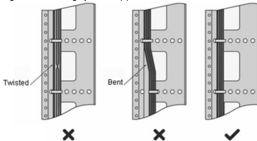
Figure 7-4 Bundling up Cables (1)
