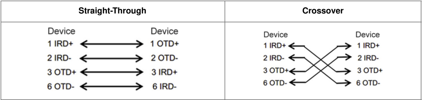
Figure 7-3 100BASE-TX Twisted Pair Connection
