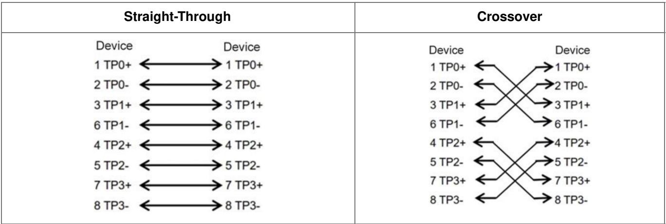
Figure 7-2 2500BASE-T/1000BASE-T Twisted Pair Connections
