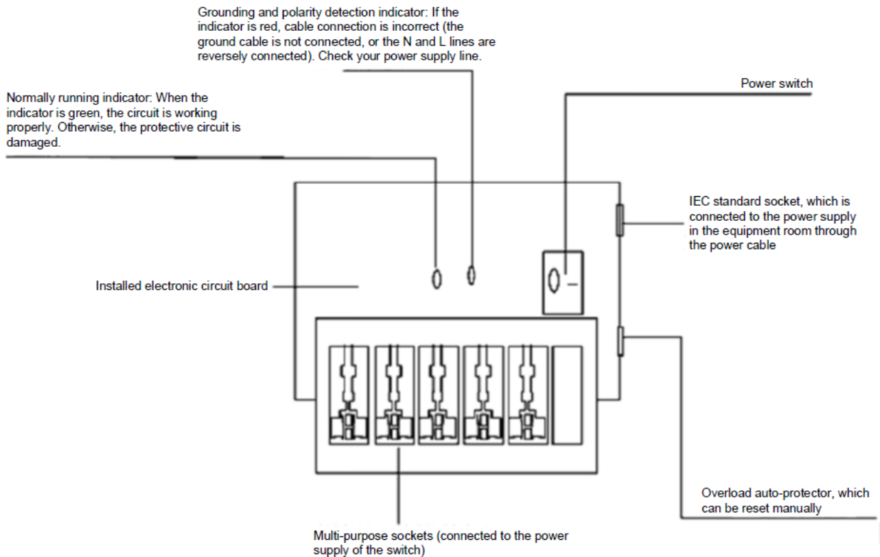
Figure 5-5 Power Arrester
