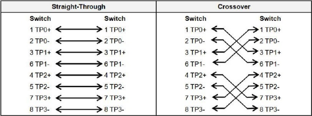
Figure 5-1 Figure 5-1 1000BASE-T Connection
