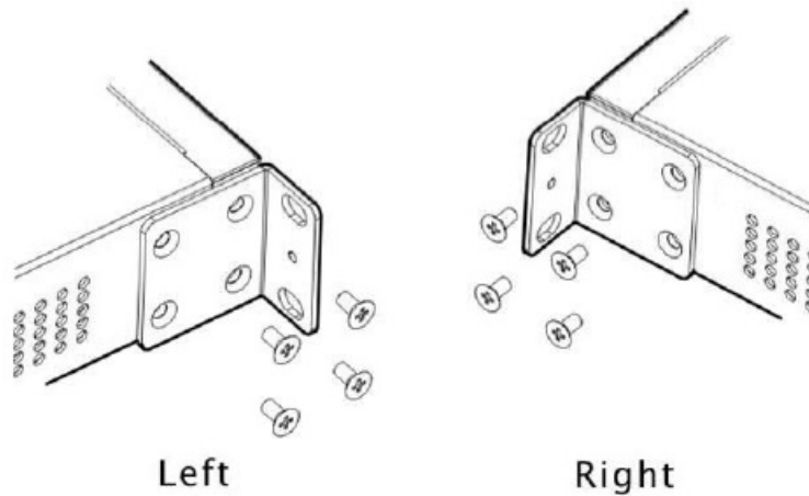
Figure 3-1 Attaching the Mounting Brackets to the Switch
