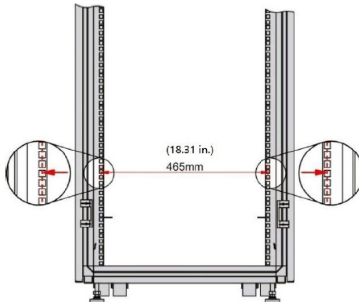
Figure 2-1 A Standard 19-inch Rack
