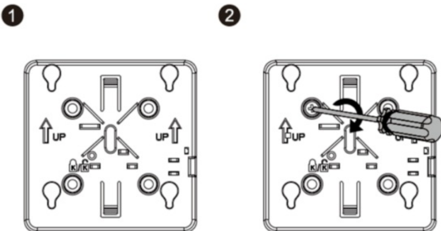
Figure 3-3 Securing the Mounting Bracket
