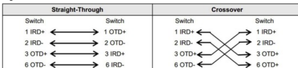
Figure 7-3 100BASE-TX/10BASE-T Connection
