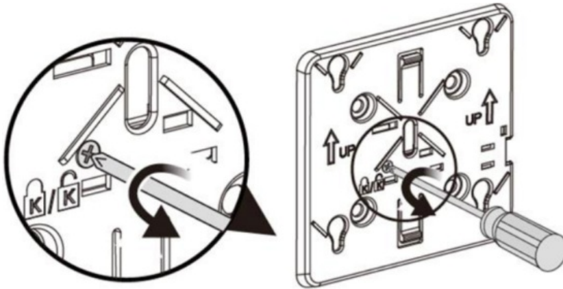
Figure 3-1 Loosening the Security Screw
