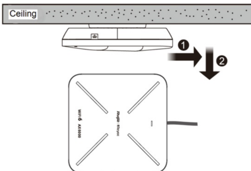
Figure 3-8 Removing the Ceiling Mount AP
