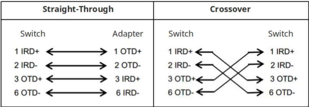
Figure 7-2 100BASE-TX/10BASE-T Twisted Pair Connections
