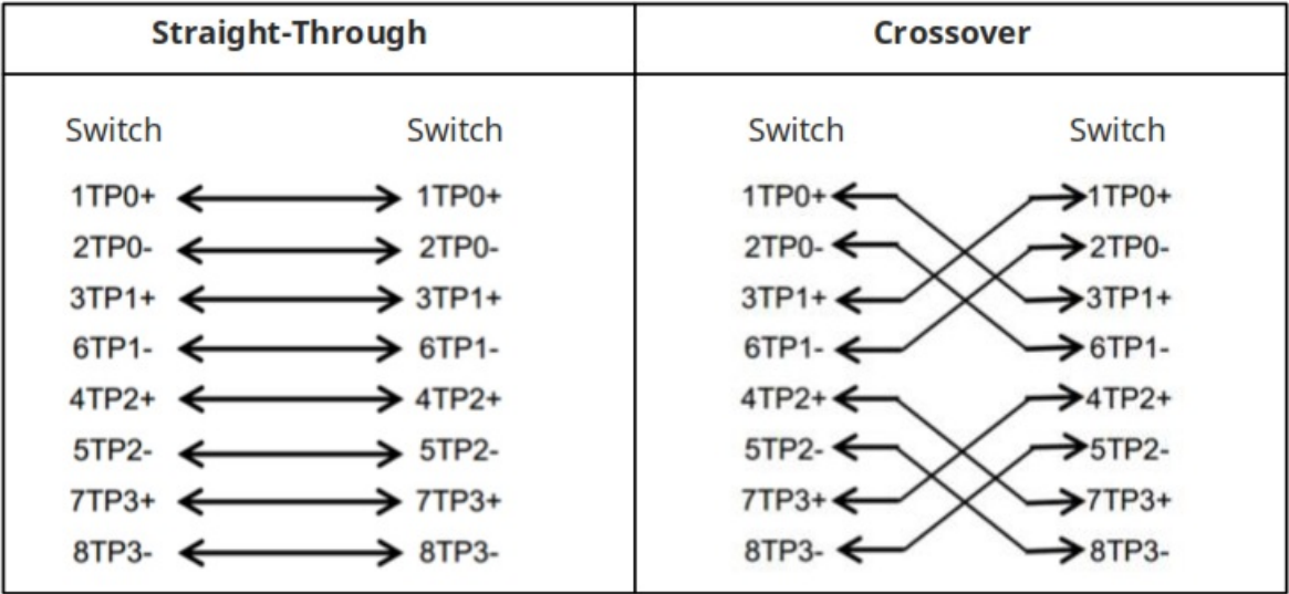
Figure 7-1 1000BASE-T Twisted Pair Connections
