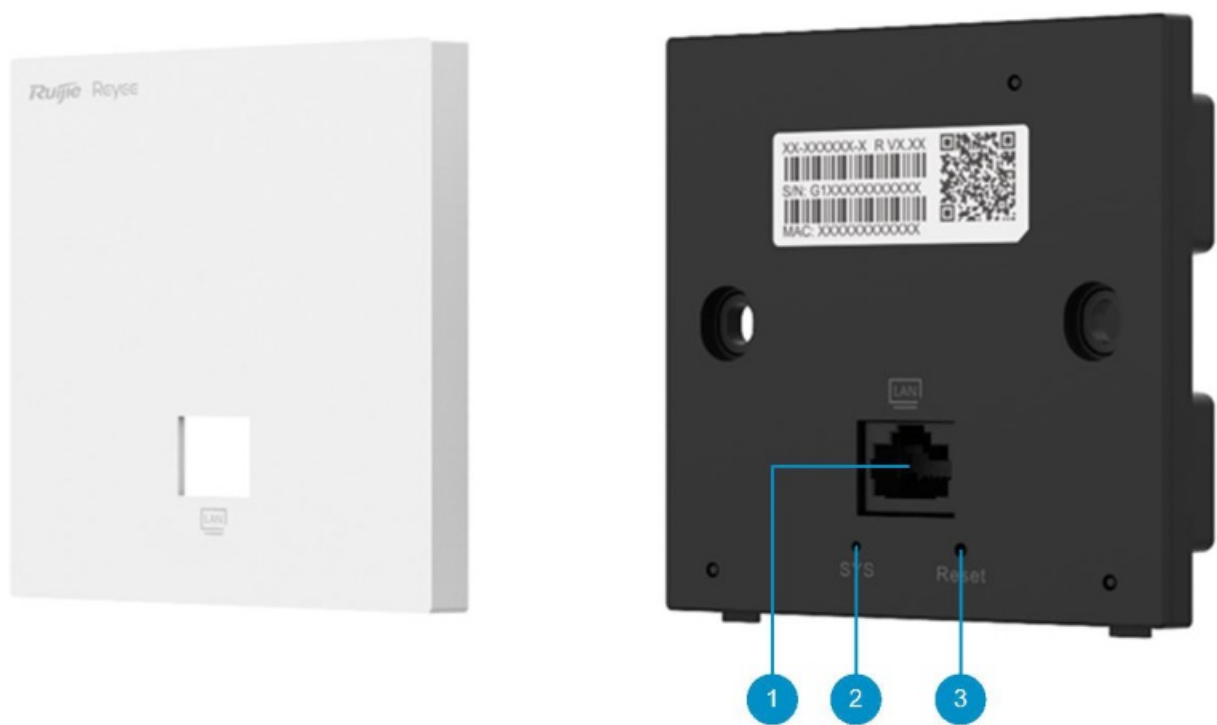
Figure 1-1 Front Panel
