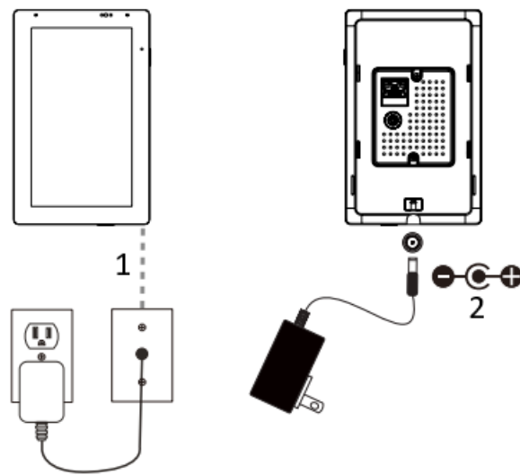
12VDC Power Supply Cabling
