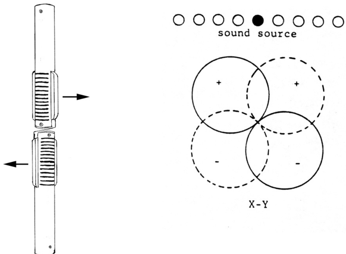
Figure 1 Classic Blumlein or "coincident" miking technique
