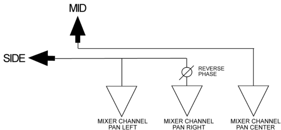
Figure 3 Typical M-S connection set-up
