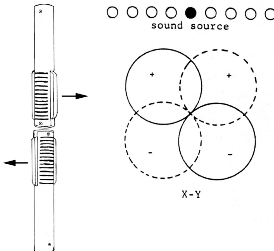
Figure 1 Classic Blumlein or coincident miking technique
