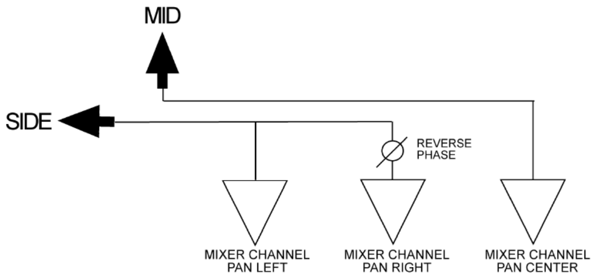
Figure 3 Typical M-S connection set-up
