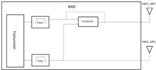
Figure 2-2 RN93xR/N GNSS Block Diagram
