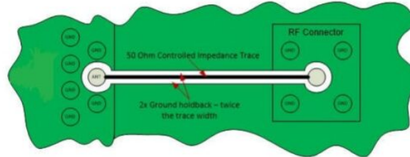
Figure 4. Antenna Microstrip Routing Example
