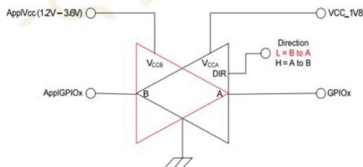
Figure 3-2 RN93xx Interface Reference Circuit
