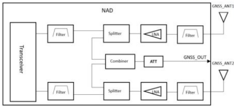
Figure 2-1 RN93xA/B GNSS Block Diagram
