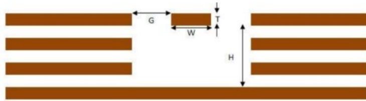
Figure 3. Coplanar Clearance Example
