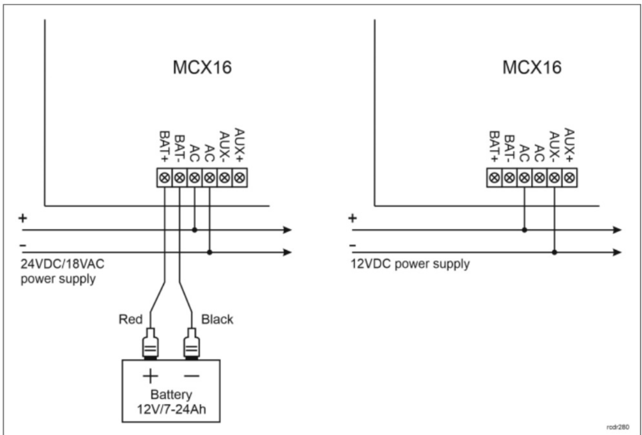
Fig. 1 MCX16 power supply
