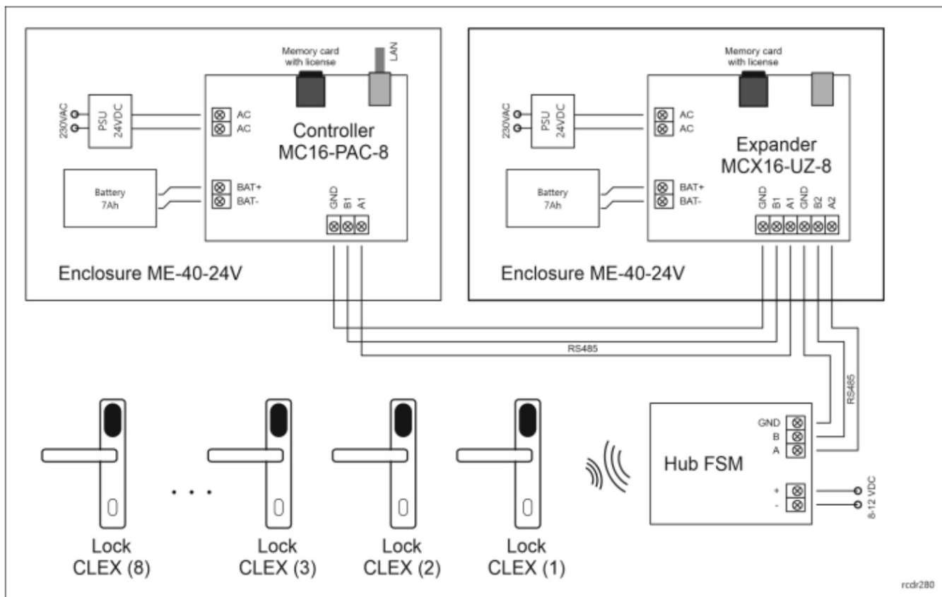
Fig. 2 Typical connection diagram
