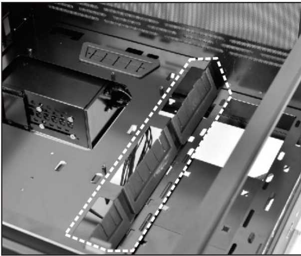
2.5" SSD / 3.5" HDD installation
