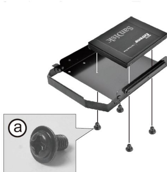
2.5" SSD installation
