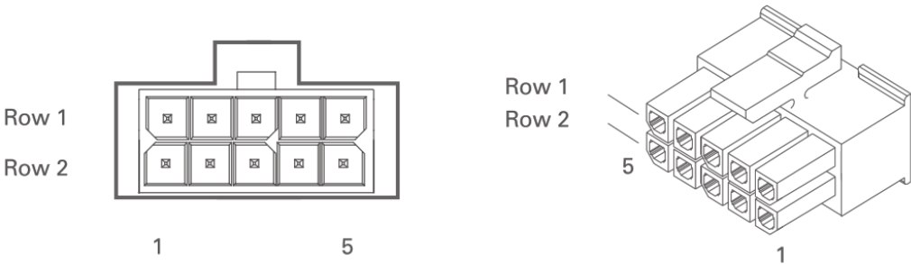
FIGURE 6. Encoder connector Each input includes a 4.7K pull-up resistor and can therefore accommodate encoders with open collector/open-drain outputs. A 1nF capacitor to ground is present on each input for noise reduction.
