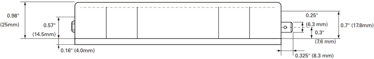
FIGURE 12. FIM2360 side view and dimensions
