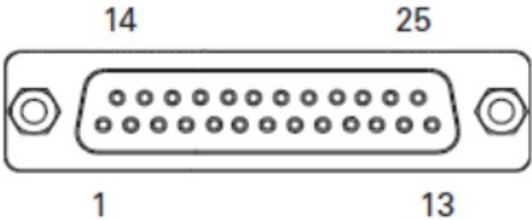
FIGURE 7. Main Connector pin locations
