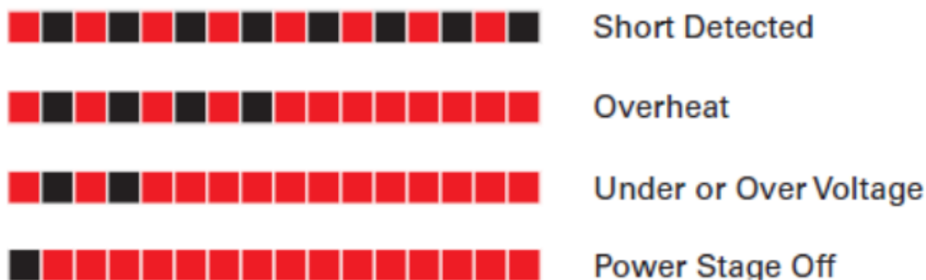
FIGURE 10. Exception or Fault Flashing Patterns
