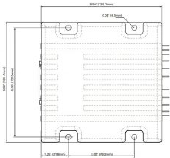
FIGURE 15. FBL2360 top view and dimensions
