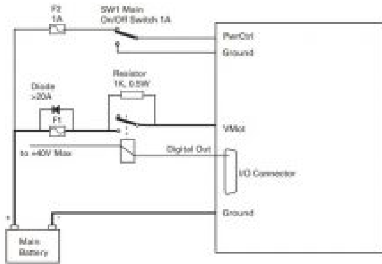
FIGURE 5. Contactor wiring diagram
