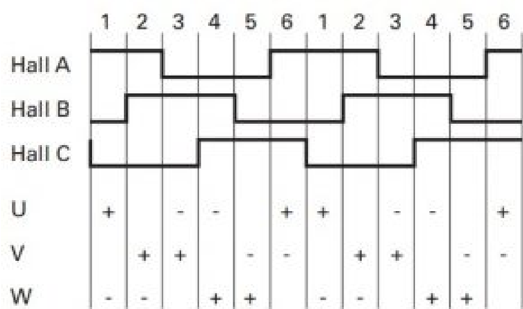
FIGURE 7. Hall Sensors sequence
