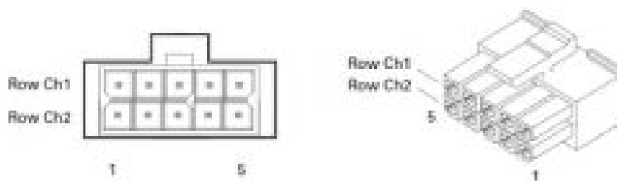
FIGURE 6. Hall Sensors connector
