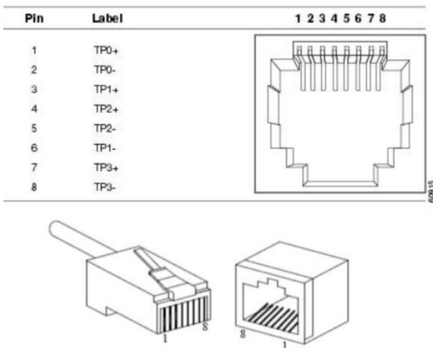
Figure 1 10/100/1000M Lan Port Pinouts
