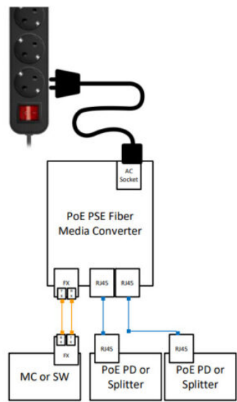
Figure: Connecting the Converter
