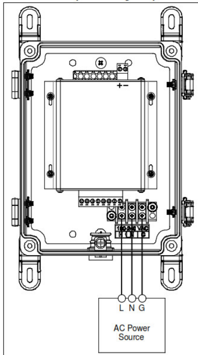
Figure 3: AC Wiring
