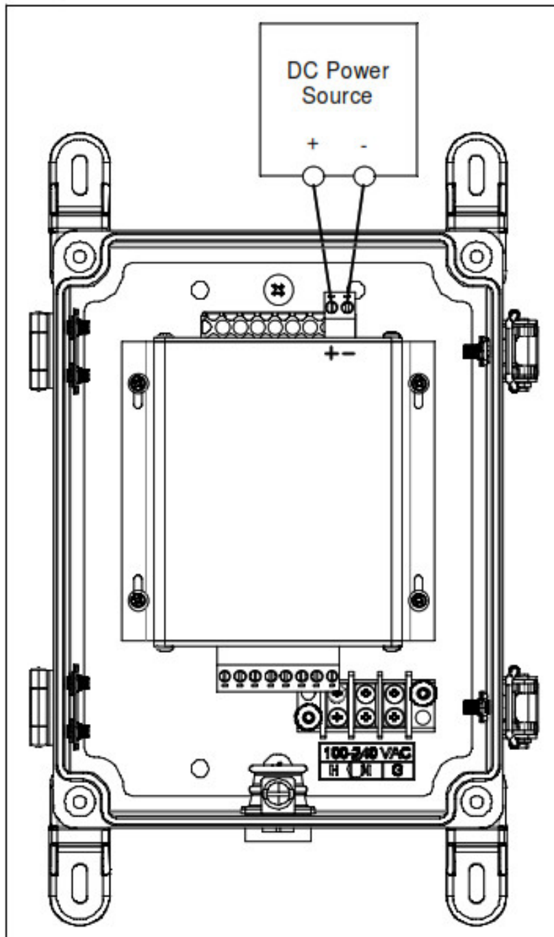
Figure 4: DC Wiring
