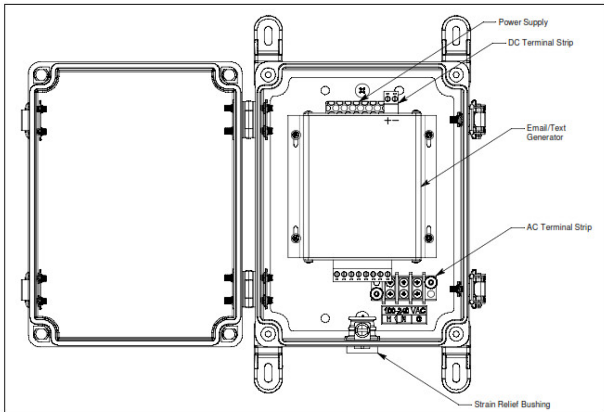
Figure 1: Component Location
