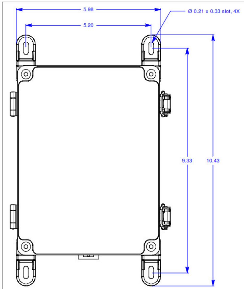
Figure 2: Dimensions
