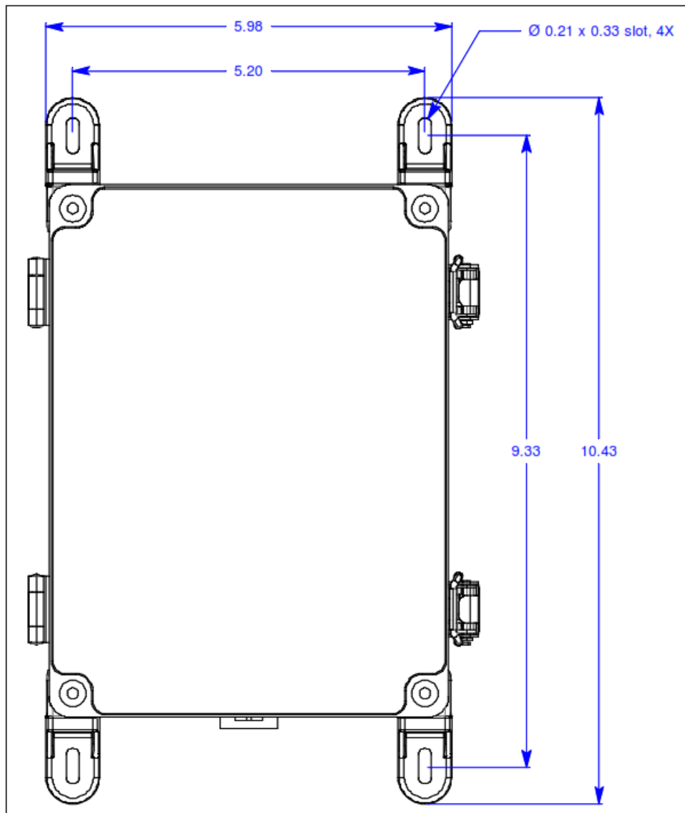
Figure 2: Dimensions
