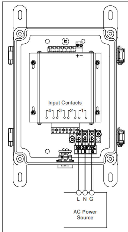
Figure 3: AC Wiring
