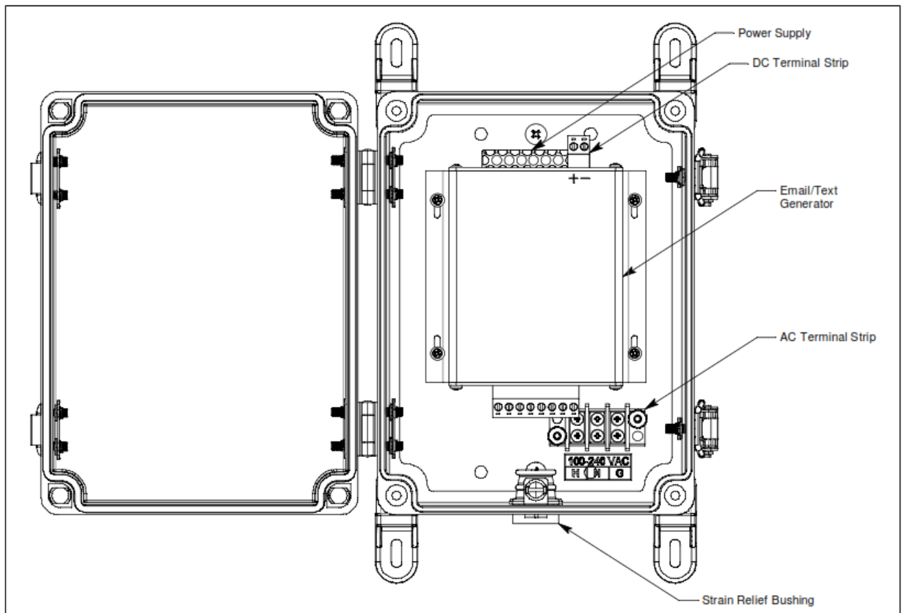
Figure 1: Component Location
