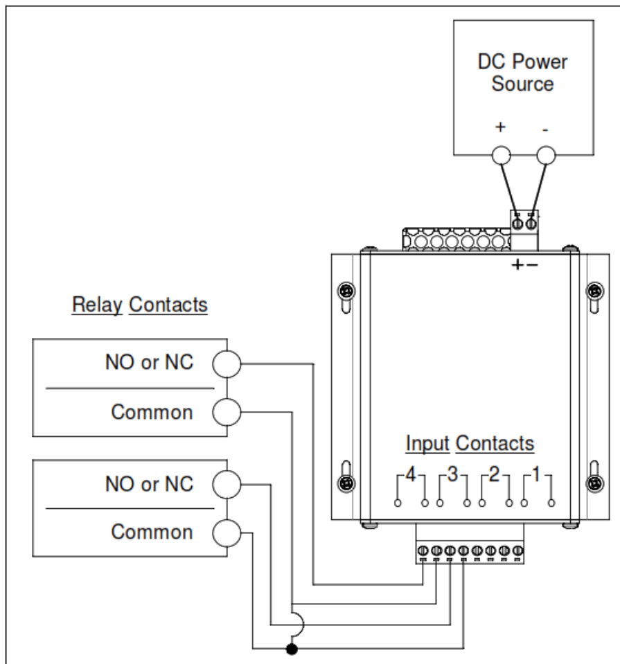
Figure 4: DC Wiring
