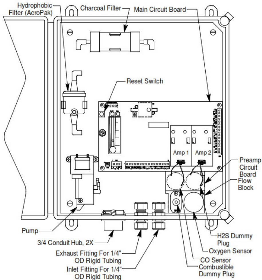
Figure 1: Sample Draw Detector Component Location
