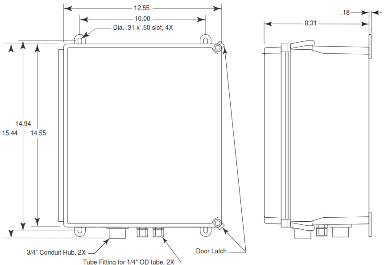
Figure 4: Mounting the Sample Draw Detector
