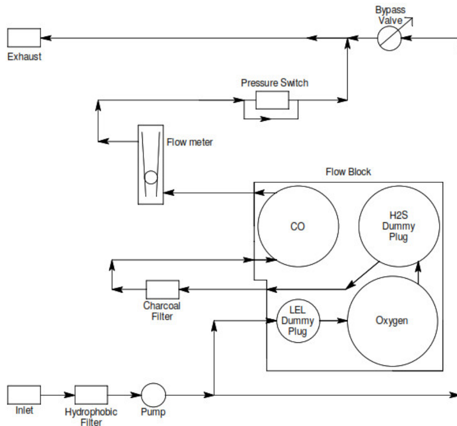
Figure 2: Sample Draw Detector Flow Diagram
