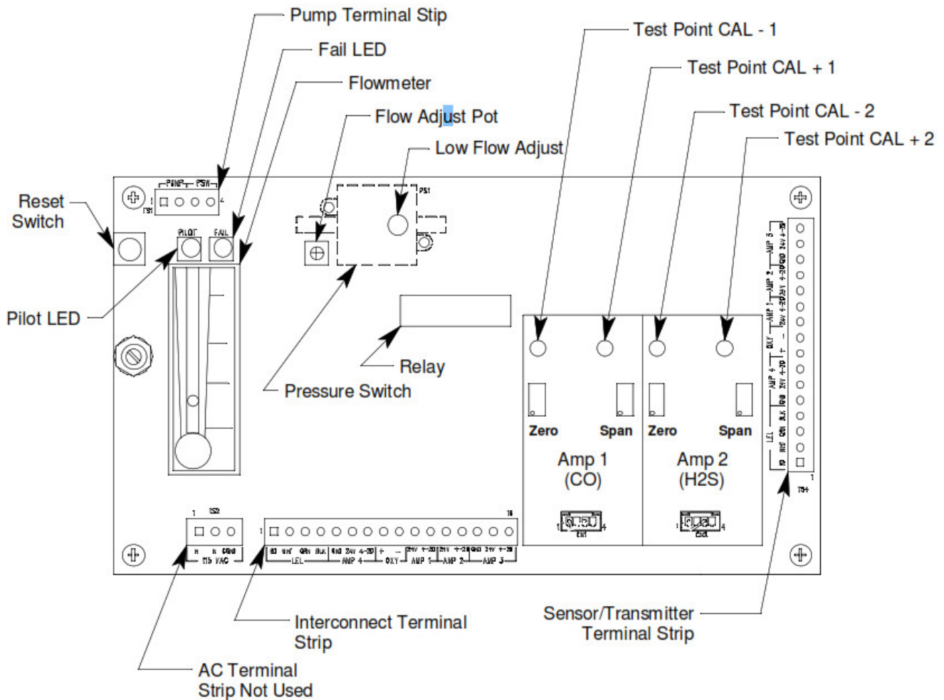
Figure 3: Main Circuit Board
