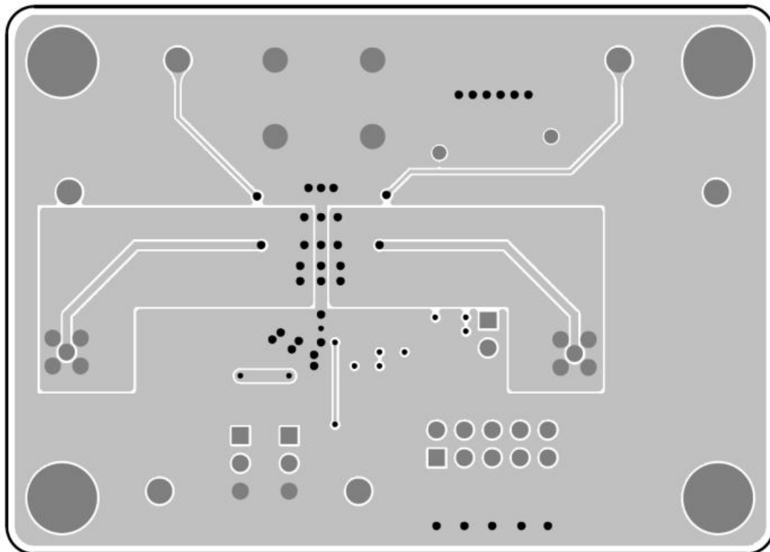
Figure 2. Bottom View (2 nd Layer)
