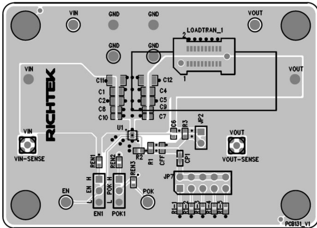
Figure 1. Top View (1 st layer)
