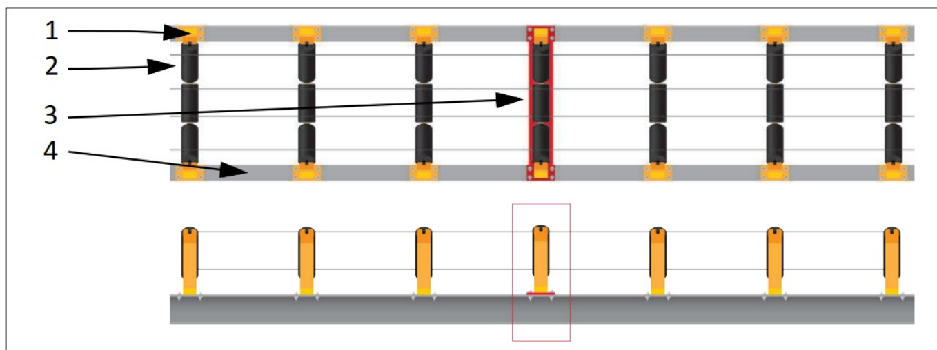
Figure 2-1. Aligned Idlers (top and side views)
