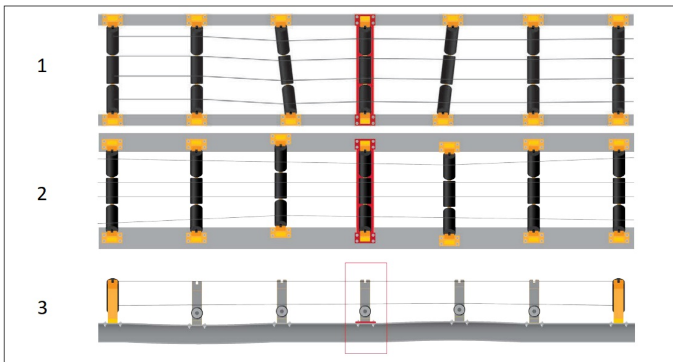
Figure 2-2. Misaligned Idlers (top and side views)
