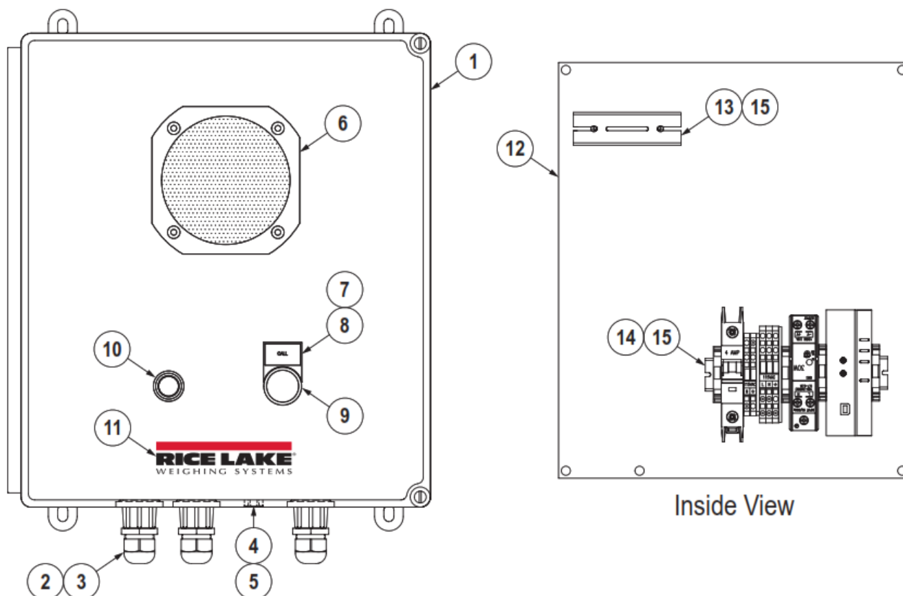
Figure 3-1. Replacement Parts Diagram
