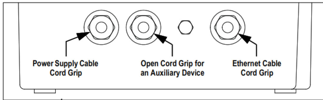
Figure 2-3. Cord Grip Assignments
