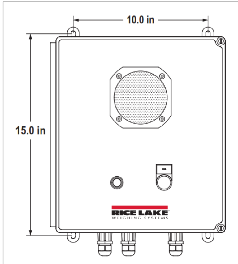
Figure 2-1. Intercom Kiosk Mounting Dimensions
