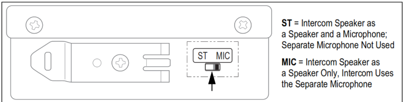
Figure 2-7. IP Endpoint Amplifier Microphone Switch
