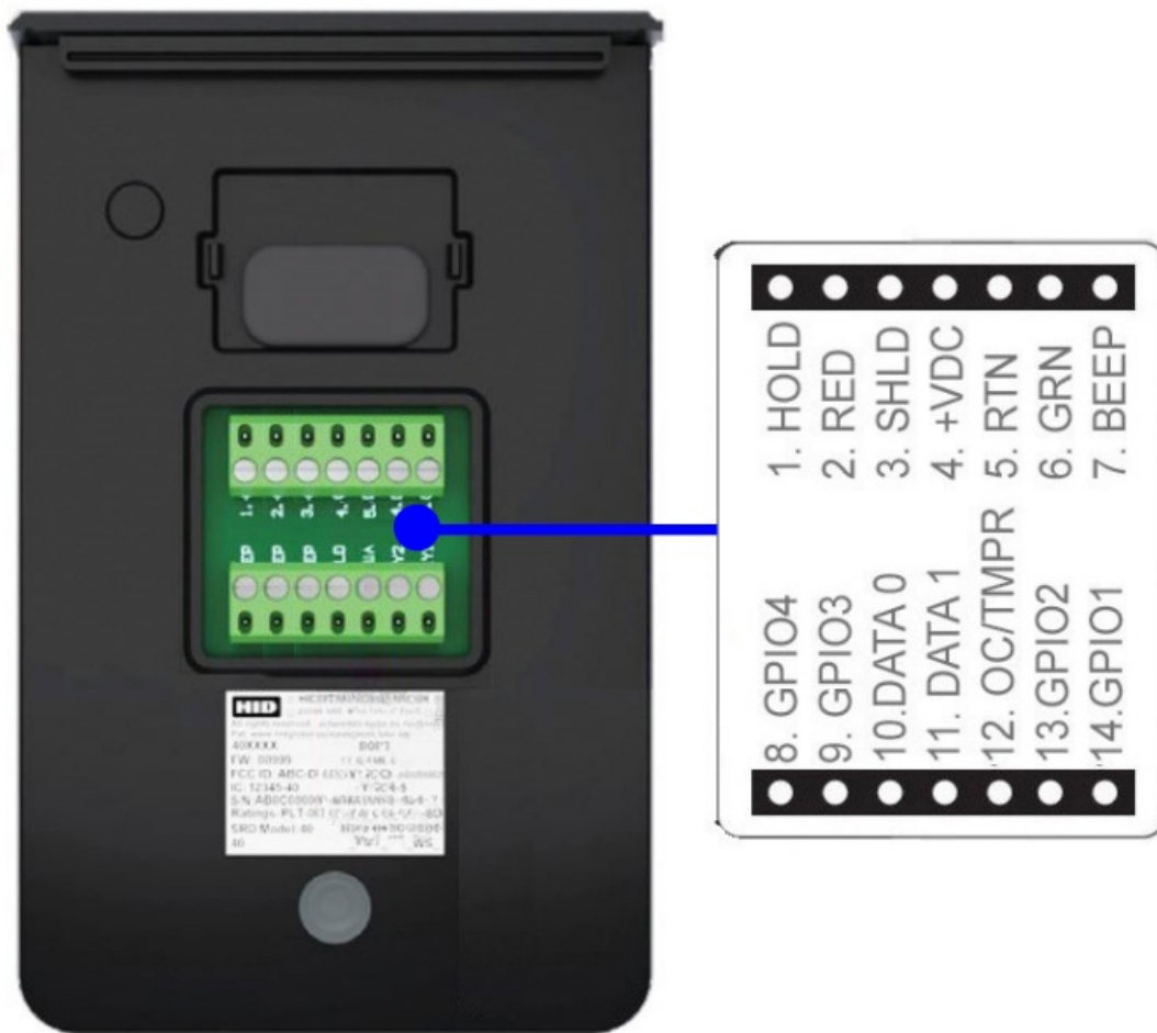
Figure 8. HID Reader Terminal Block Pinout
