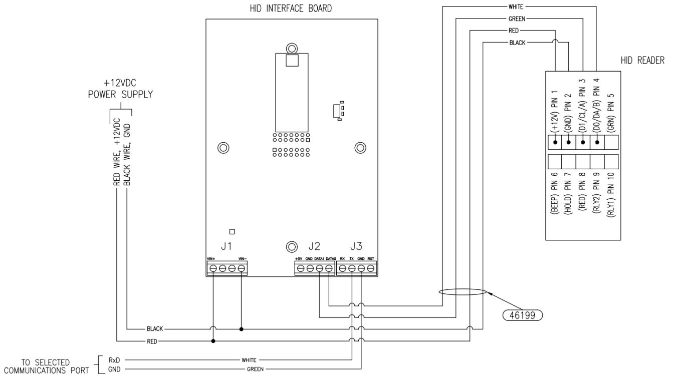
Figure 5. Interface Board Wiring Diagram
