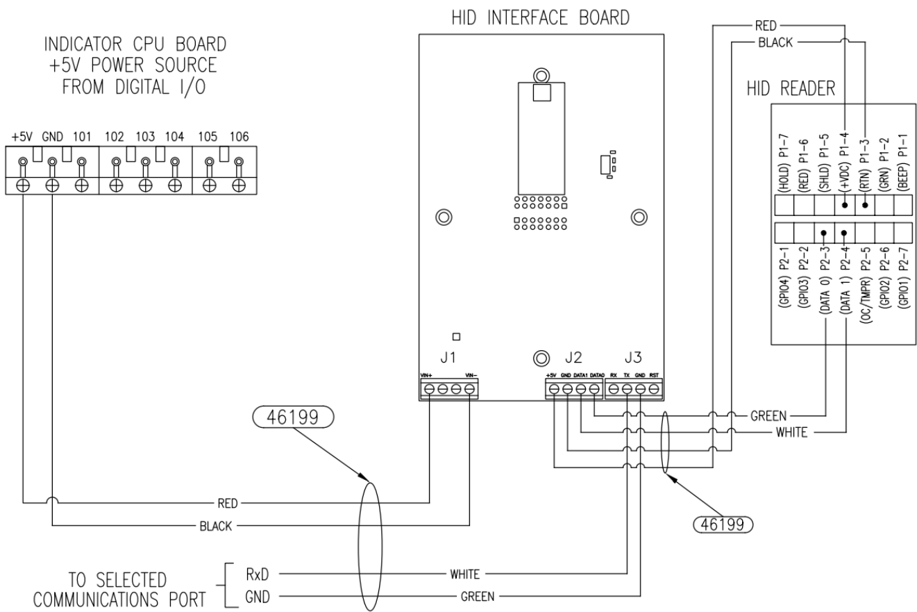
Figure 7. Interface Board Wiring Diagram
