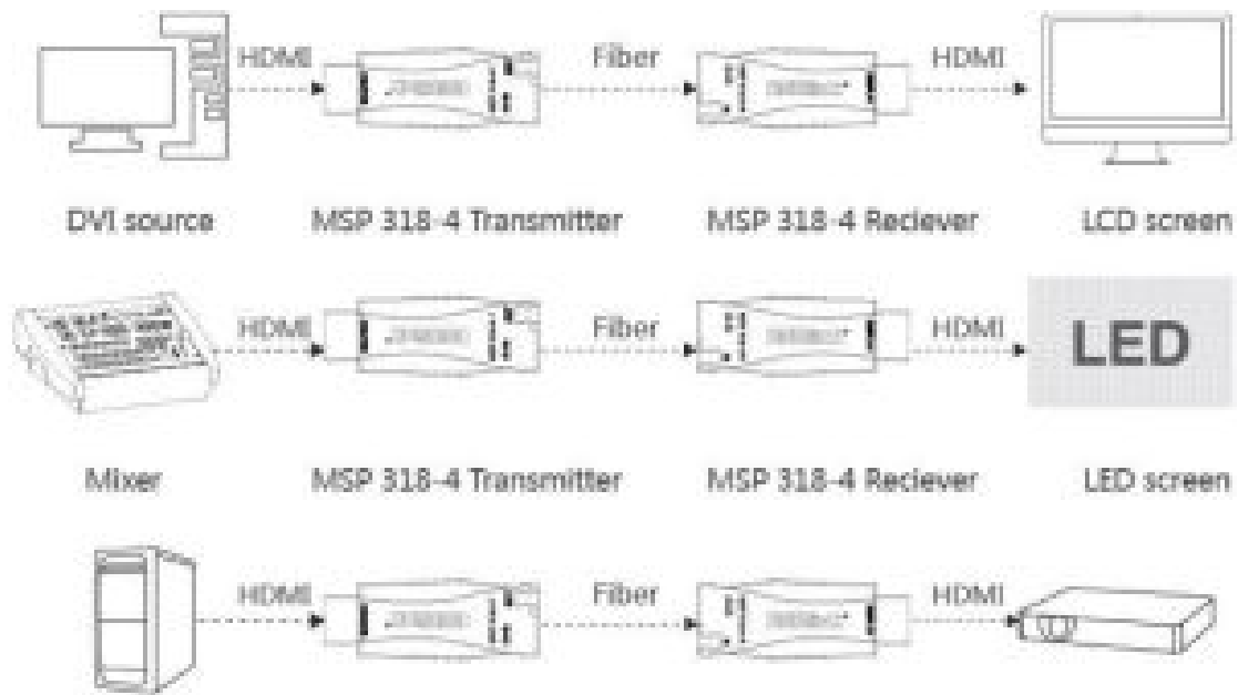
MSP 318-4 System Connection Diagram
