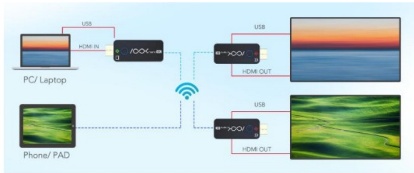
ASK nano System Connection Diagram 2
