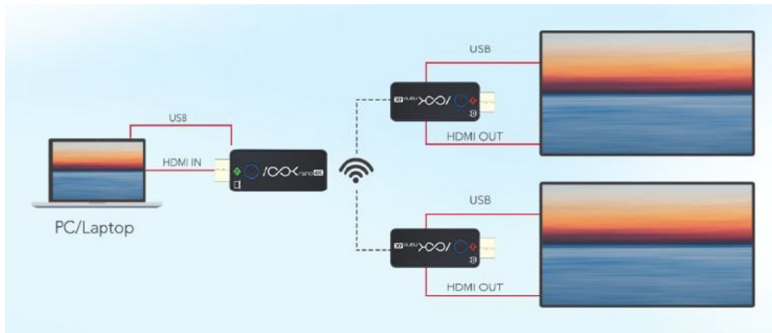
ASK nano System Connection Diagram 1
