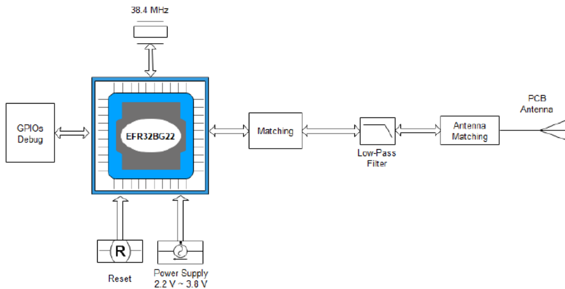
Figure 1. Functional Block Diagram of RF-BM-BG22B1
