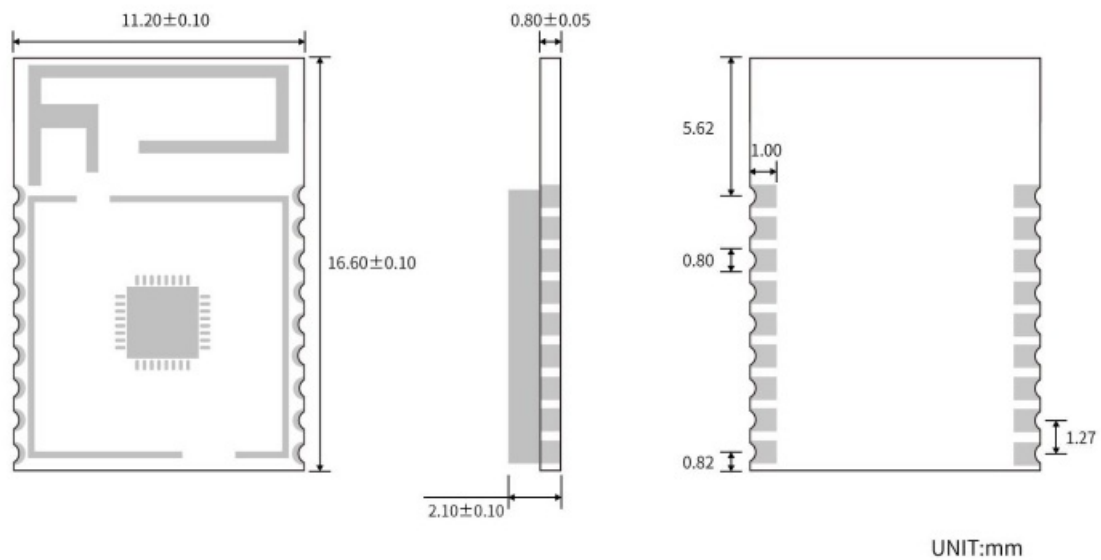
Figure 5. Recommended PCB Footprint of RF-BM-BG22B1 (mm)
