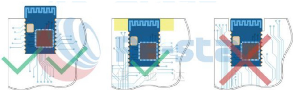
Figure 6. Recommendation of Antenna Layout
