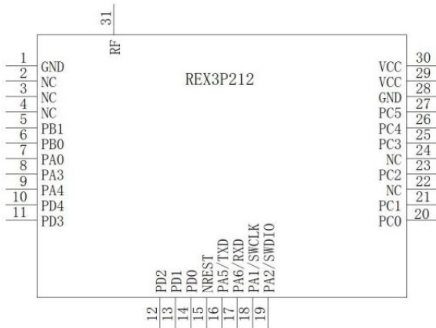
Figure 2-3 Pin configuration diagram
