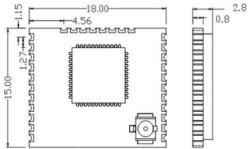
Figure 2-1 Dimensions
