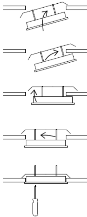
Installing in Ceiling
