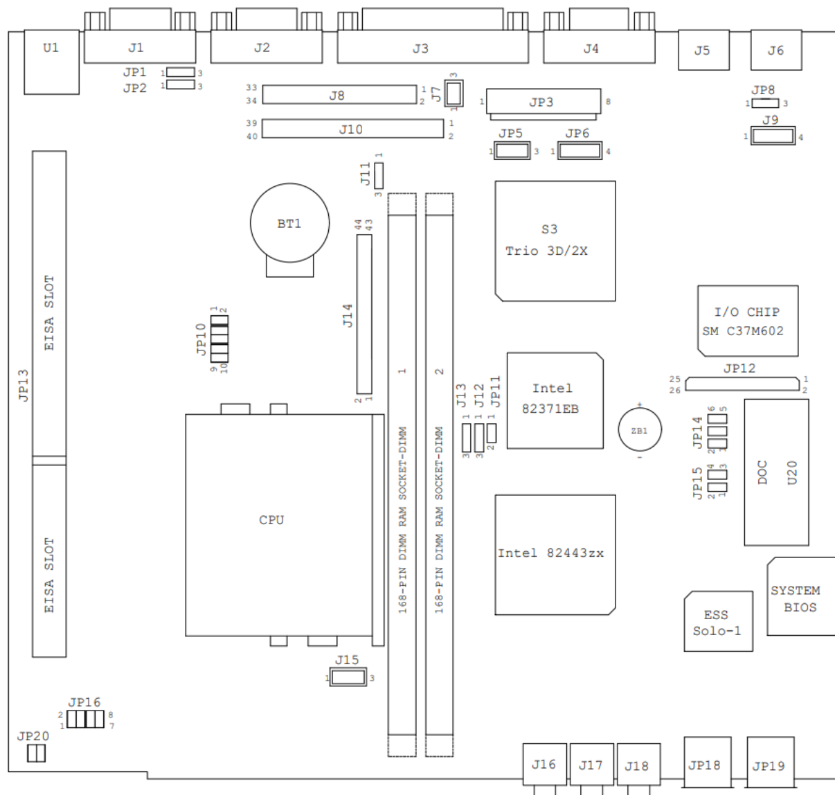
Memory configuration for “B62 V1.X” main board
