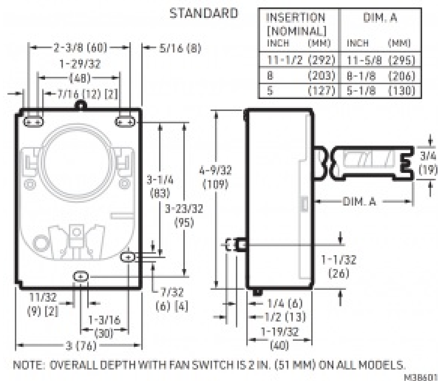
Fig. 1. MOUNTING DIMENSIONS IN in. [mm IN BRACKETS].
