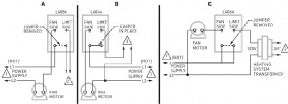
Fig. 10. L4064T,W,Y 3-WIRE LINE VOLTAGE HOOKUP.
