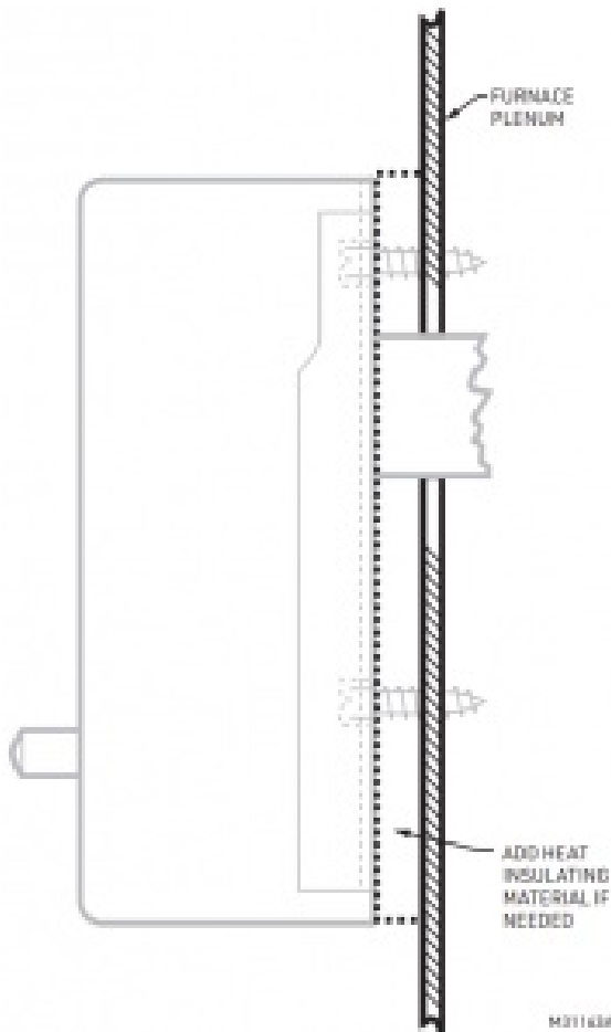
Fig. 3. SURFACE MOUNTING FOR L4064. THE L4064C AND D REQUIRE A 1-1/2 in. [38.1 mm] HOLE FOR ELEMENT INSERTION; ALL OTHER MODELS REQUIRE A 13/16 in. [20.6 mm] HOLE.
