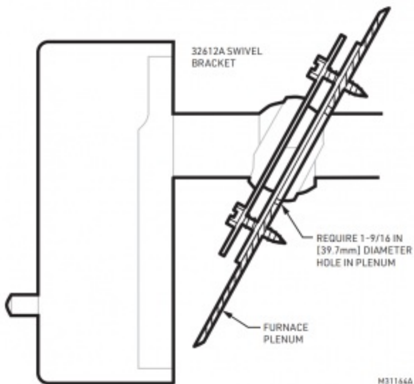
Fig. 4. SWIVEL MOUNTING. REQUIRES A 1-9/16 in. [39.7 mm] DIAMETER HOLE FOR ELEMENT INSERTION.
