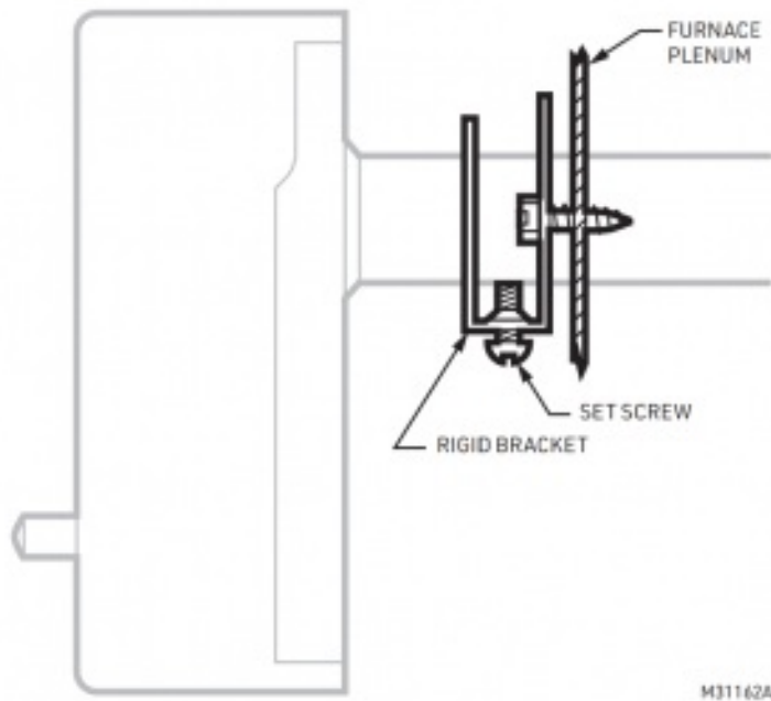
Fig. 5. RIGID BRACKET MOUNTING REQUIRES A HOLE 13/16 in. [20.6 mm] DIAMETER FOR ELEMENT INSERTION.
