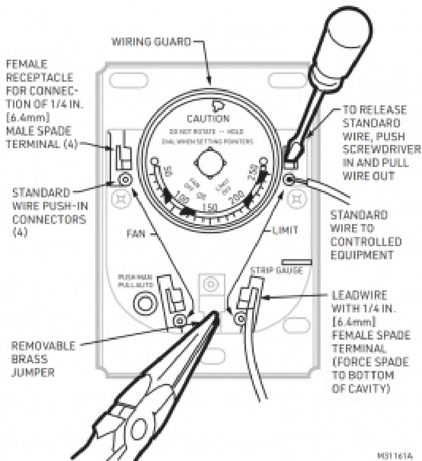
Fig. 9. LOCATION OF WIRING CONNECTIONS.
