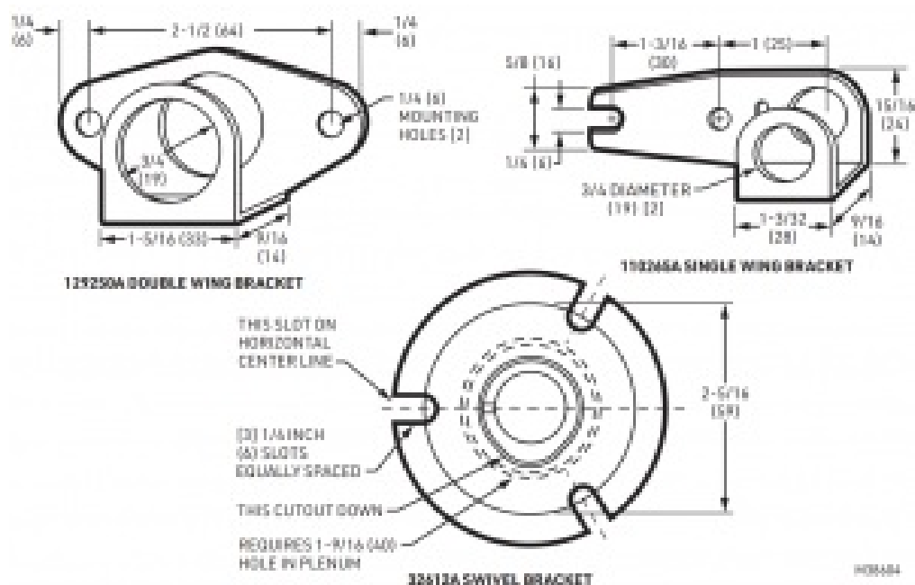
Fig. 2. MOUNTING DIMENSIONS IN in. [mm IN BRACKETS] OF BRACKETS.
