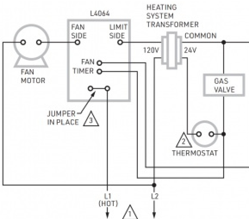
Fig. 9. LOCATION OF WIRING CONNECTIONS.
