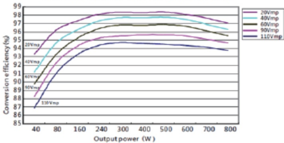
MPPT 12V conversion efficiency (12V battery)
