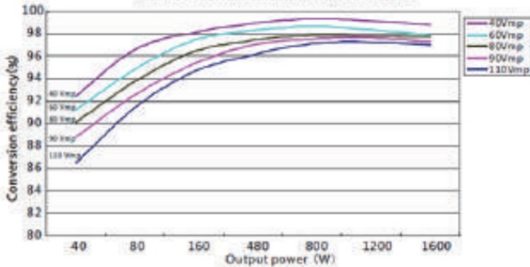
MPPT 24V conversion efficiency (24V battery)
