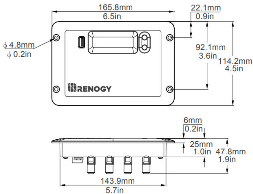
Adventurer Controller
