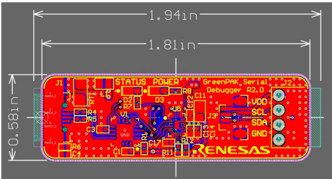
Figure 2: PCB
