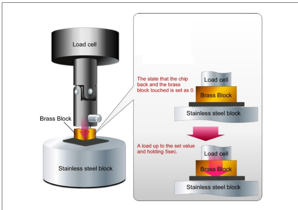
Figure 1.1 Stress testing machine image
