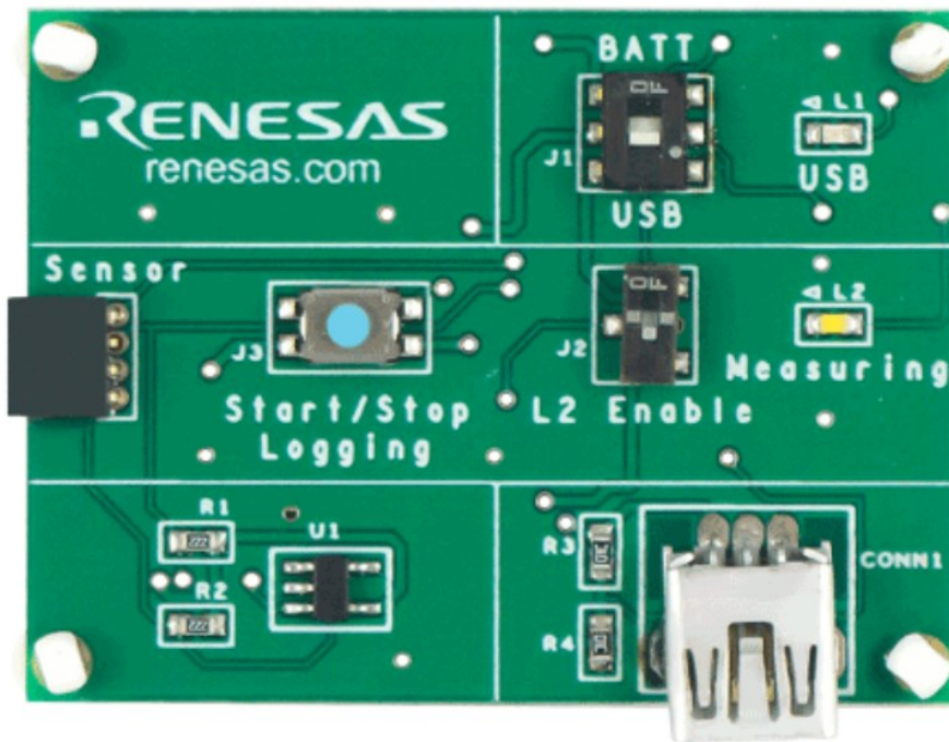
Figure 1. HS4000-EVK Evaluation Kit
