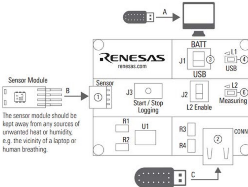
Figure 3. Evaluation Kit Connections
