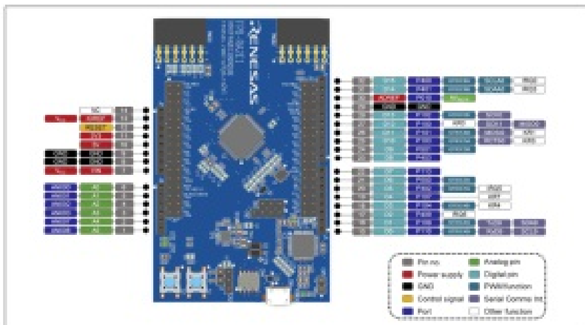
Figure 2. FPB-RA2E1 Arduino Interface
