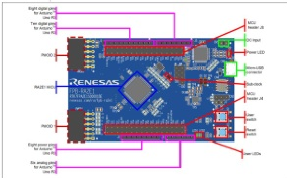
Figure 1. FPB-RA2E1 Board Layout
