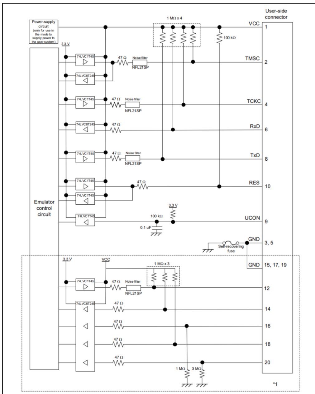
Figure 2-7 Internal Circuits of the E2 (Rev. D)
