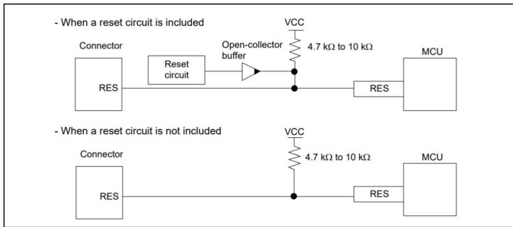
Figure 2-4 Connection of the RES Pin
