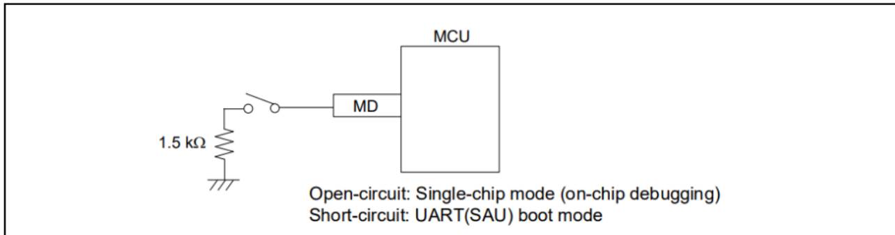
Figure 2-5 Connection of the MD Pin
