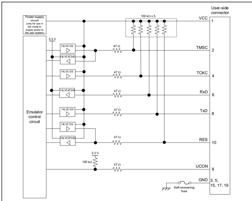
Figure 2-8 Internal Circuits of the E2 Lite
