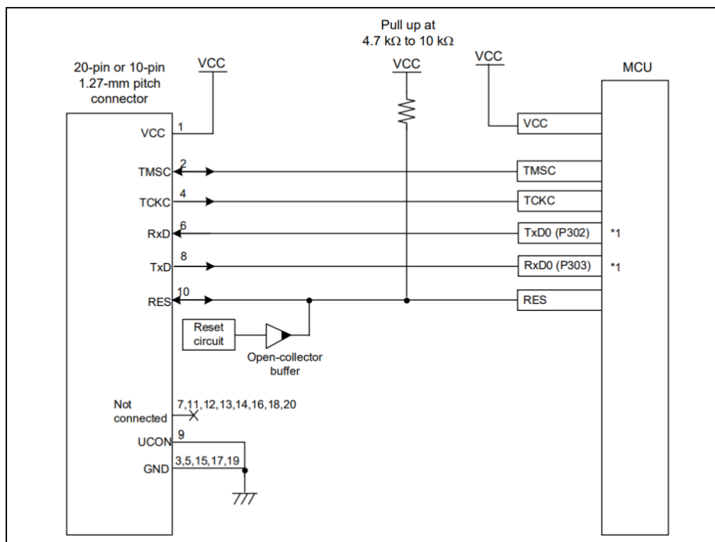
Figure 2-3 Example of a Connection through cJTAG Interfaces
