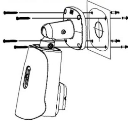
Figure 3-1 Installing bracket
