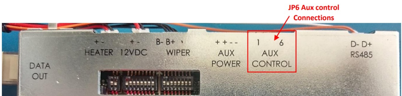
Fig 22 JP6 Aux control connections
