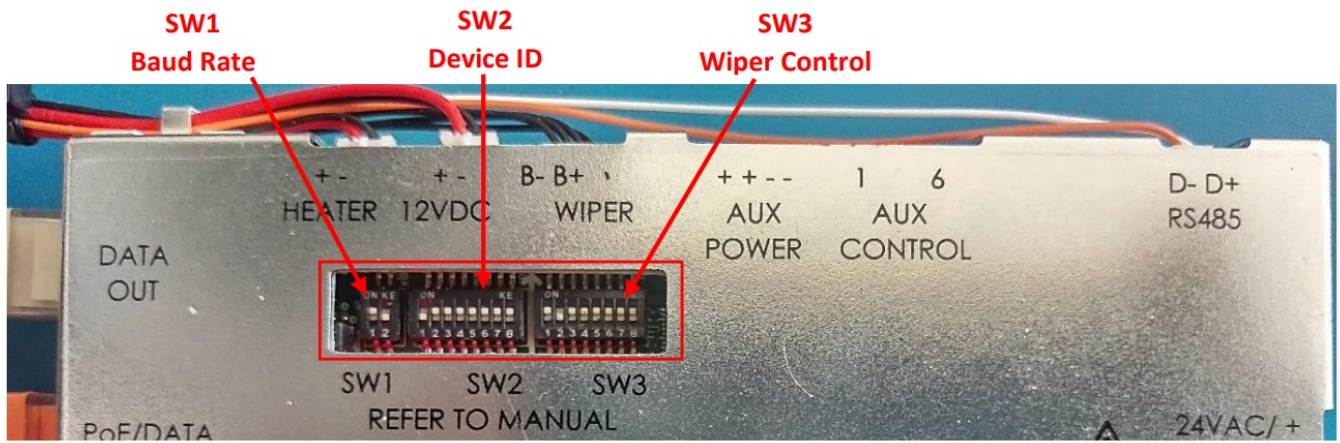
Fig 20 CHAT™ board, showing DIP switch blocks
