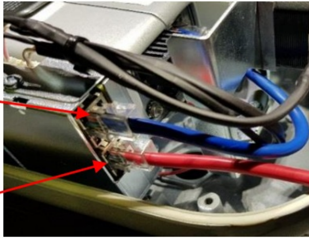
Fig 19 CHAT™ board, showing PoE+ (802.3at) input & data output
