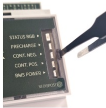
Figure 2: Opening the front cover
