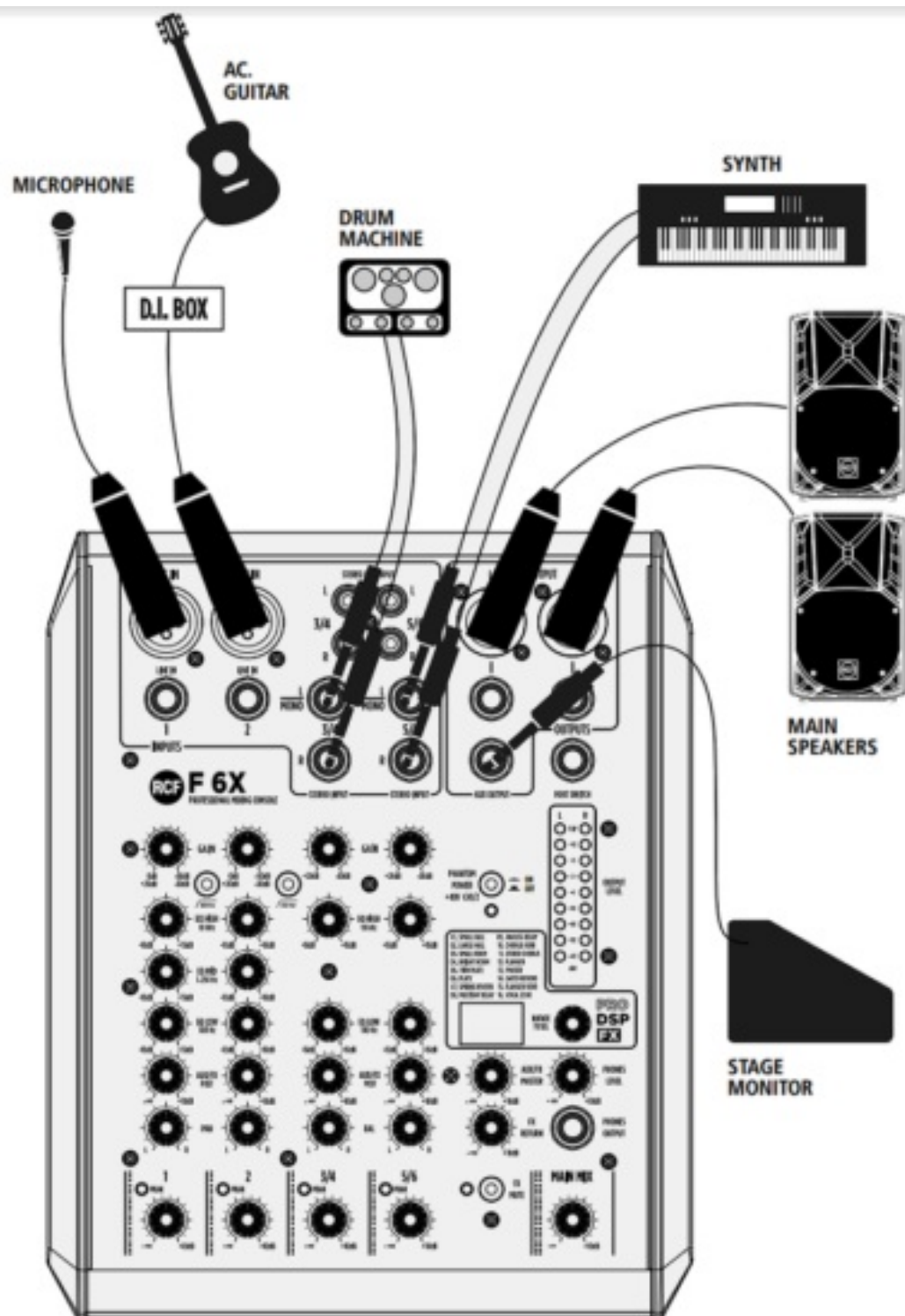
F 6X BLOCK DIAGRAM / SCHEMA A BLOCCHI
