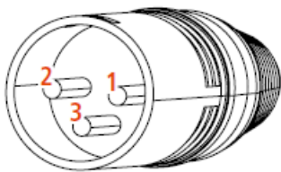
MALE XLR CONNECTOR Balanced wiring
