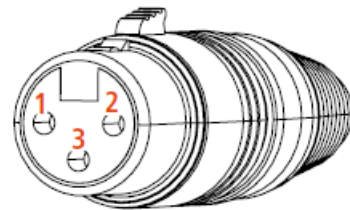
FEMALE XLR CONNECTOR Balanced wiring
