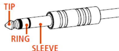
TRS CONNECTOR Balanced mono wiring
