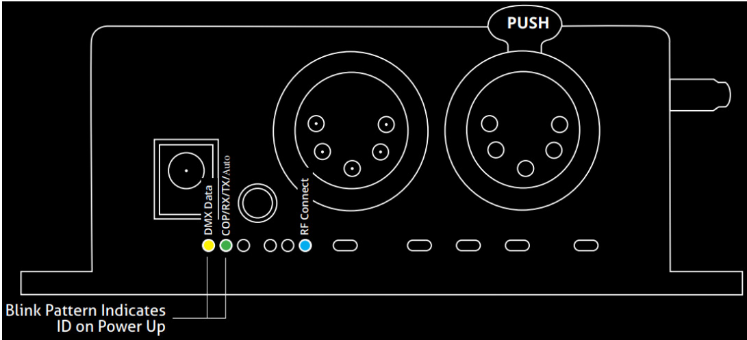
RC4Magic Indicator LEDs After Power-Up
