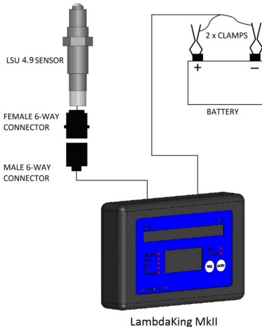
Figure 3 – Connection Schematic
