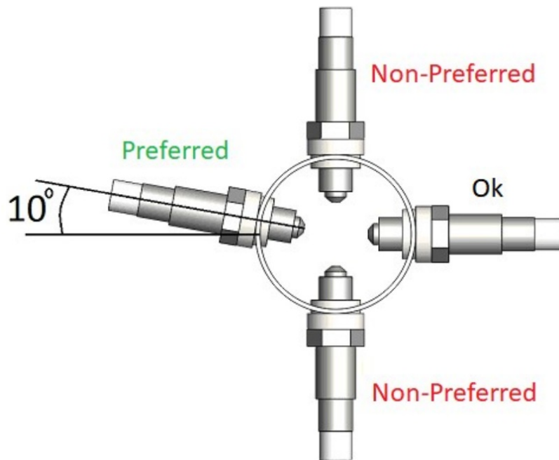
Figure 4 – Sensor Placement
