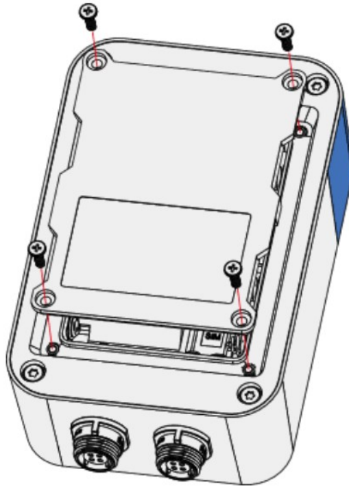
Figure 1: Removing the back cover
