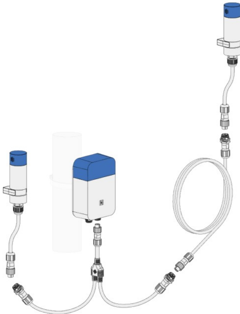
Figure 17: Connection via splitter and extender
