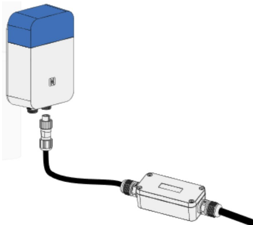
Figure 22: Connection the Probe IO to the Hub
