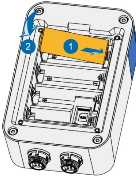
Figure 3: Fitting the batteries
