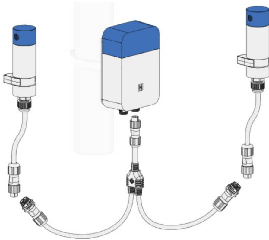
Figure 16: Connection via a splitter
