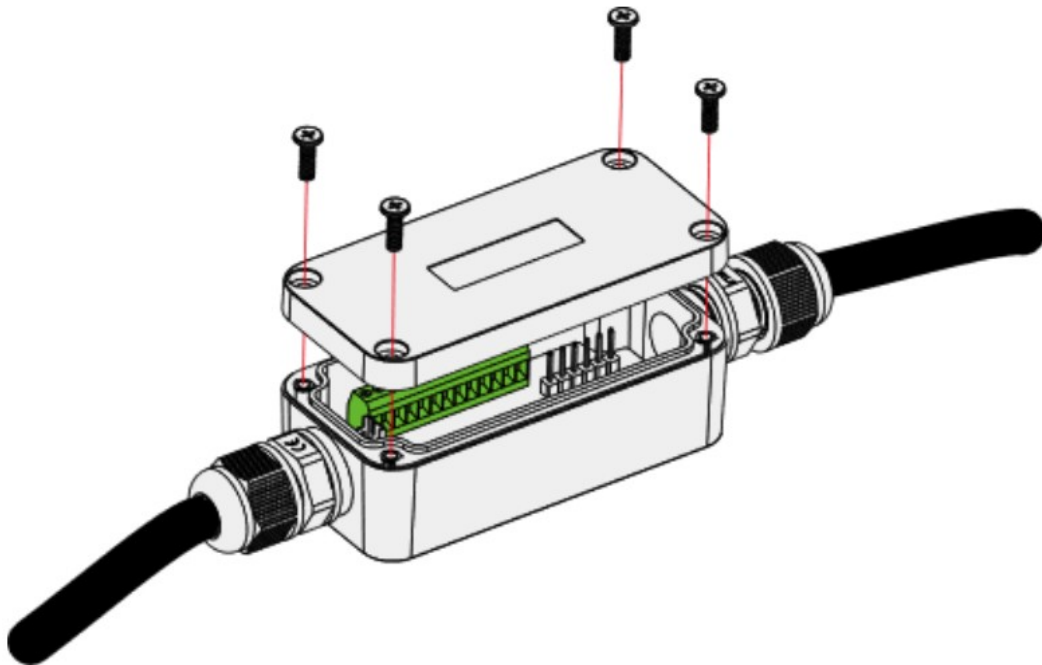
Figure 21: Closing the Probe IO
