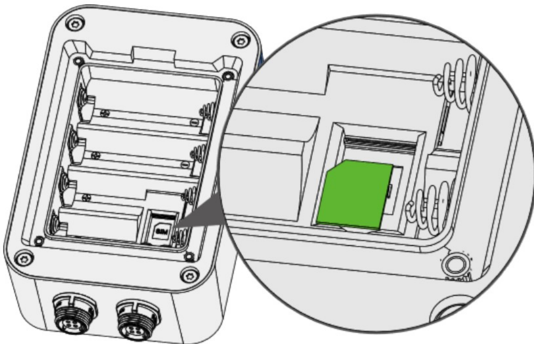
Figure 2: Inserting the SIM card
