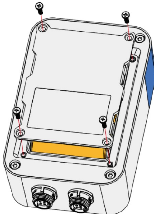
Figure 4: Closing the back cover
