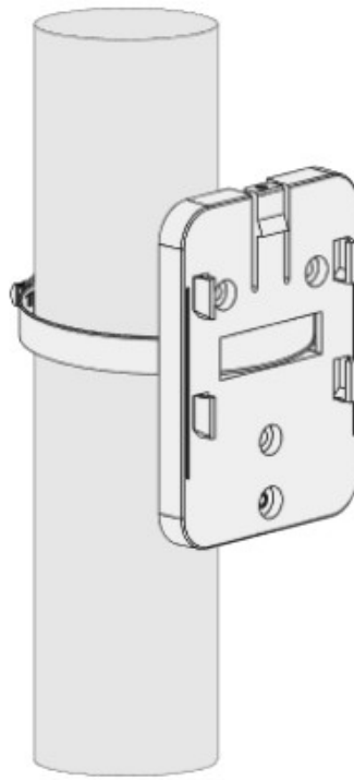
Figure 7: Installing the bracket on a pole
