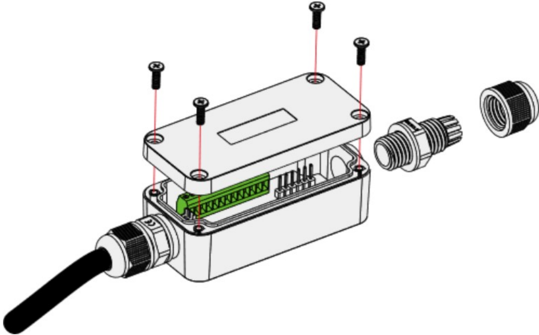
Figure 18: Removing the lid
