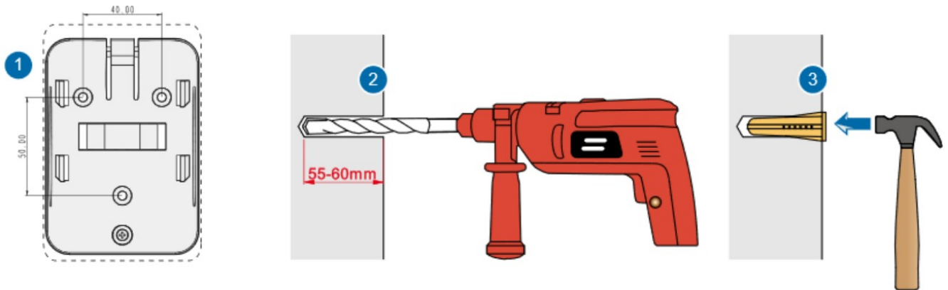
Figure 5: Drilling the wall
