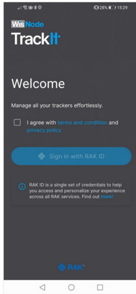
Figure 13: Welcome screen
