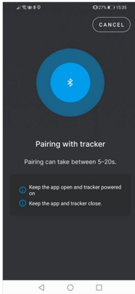
Figure 25: Pairing screen
