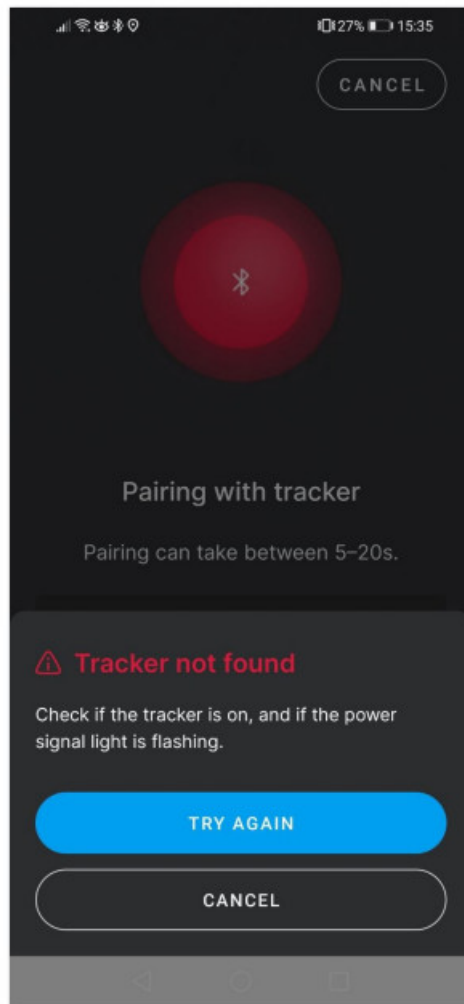
Figure 17: Pairing screen
