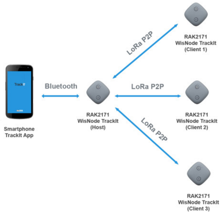
Figure 12: P2P mode
