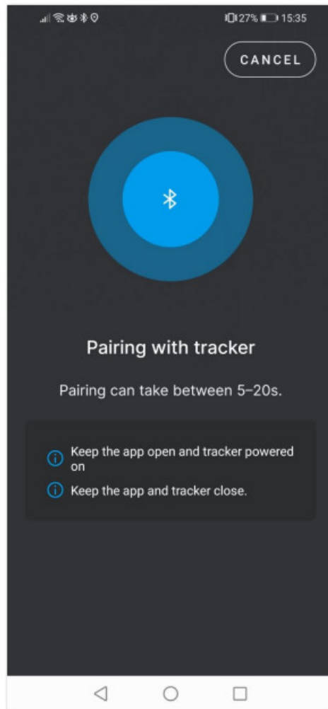
Figure 6: Pairing screen
