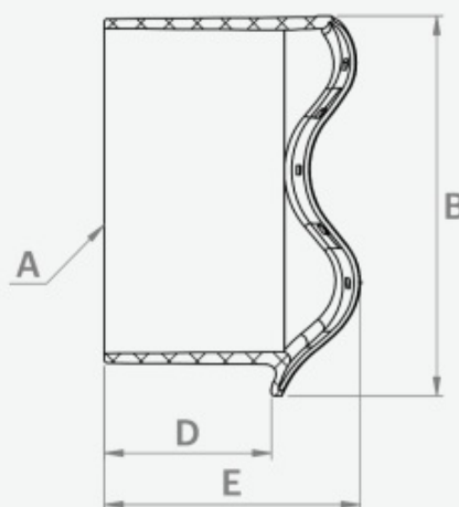
SECTION VIEW
