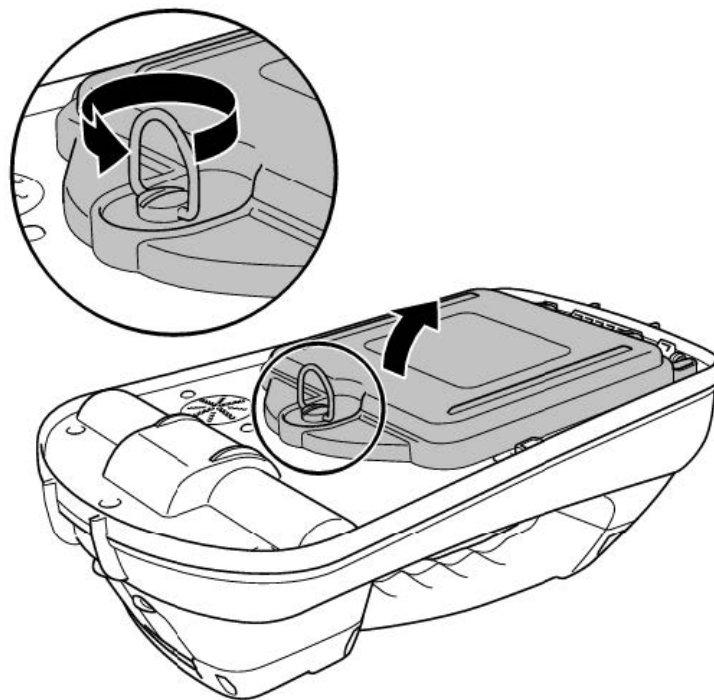
Figure 4.9: Opening the battery compartment
