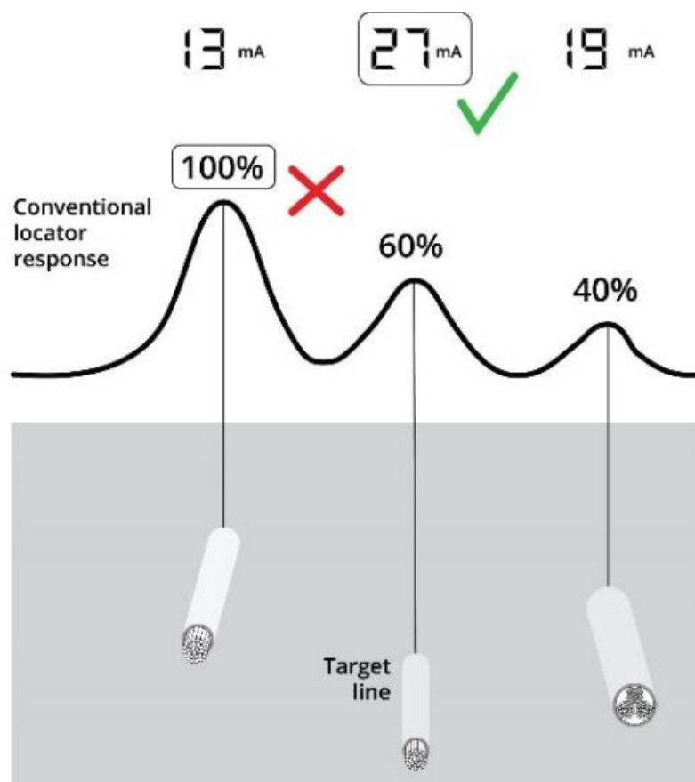
Figures 6.4 – 6.6 Taking current readings
