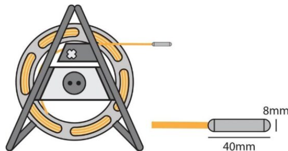
Figure 9.10: FlexiTrace
