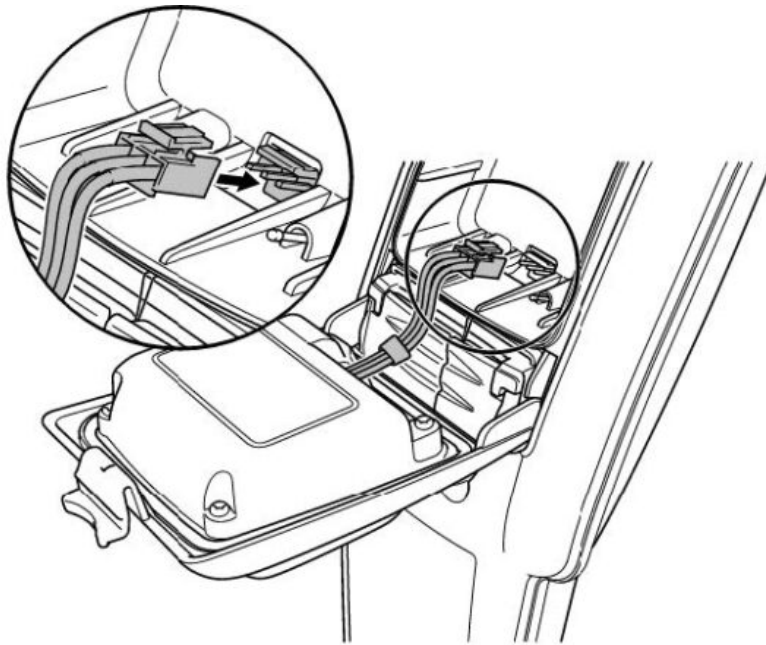
Figure 4.7 Connecting the Li Ion lead
