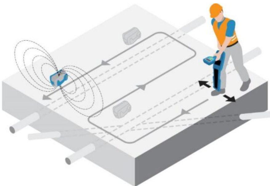
Figure 5.6 Nulling Out – Single person sweep
