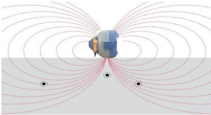
Figure 5.6 Nulling Out effect
