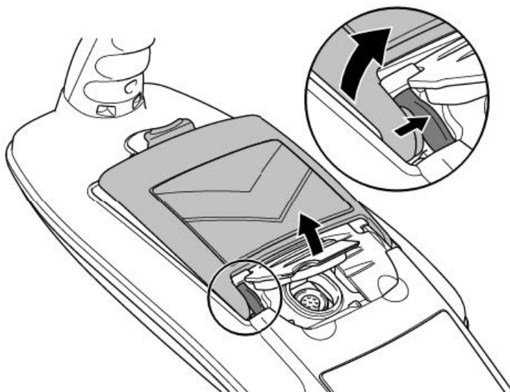
Figure 4.4 Press the retaining latch inwards
