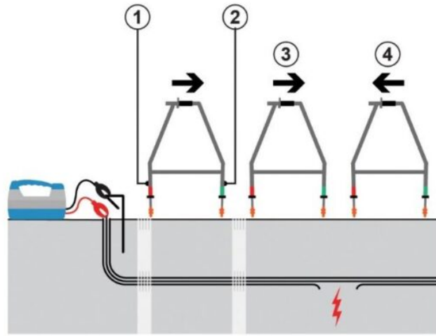
Figure 8.1: Cable sheath fault-finding
