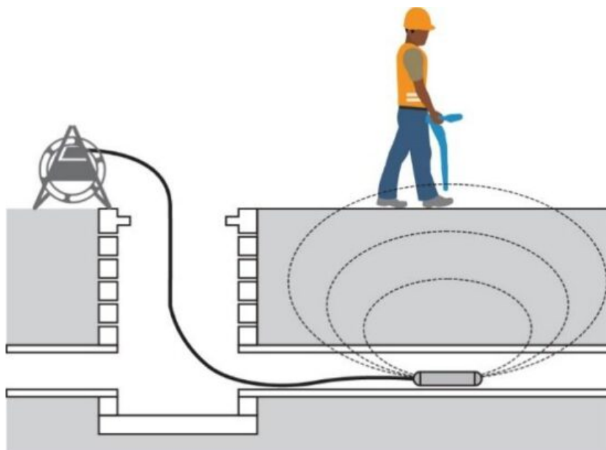
Figure 9.7 Sonde deployment
