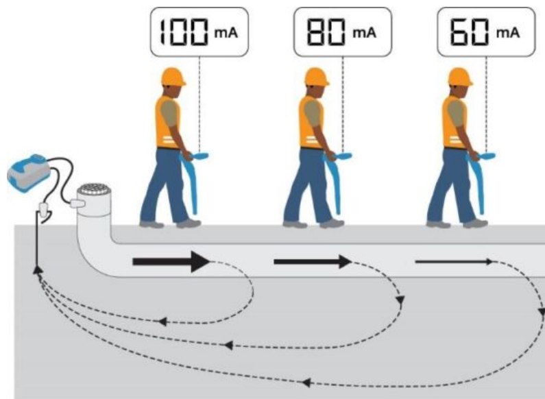
Figure 6.7: Current readings using transmitter signals
