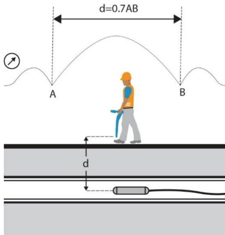
Figure 9.9: Calculating sonde depth
